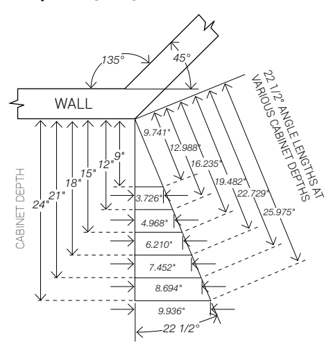
22 1/2° ANGLE CHART
