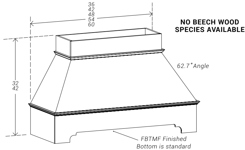
Overall Width Chart for Standard & Valance Compound Angle Hoods
