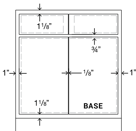
STANDARD OVERLAY - BUTT DRAWER FRONTS
