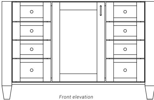
Front elevation
