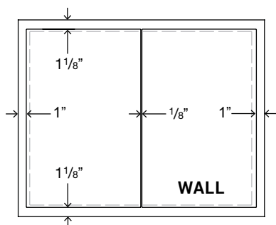
STANDARD OVERLAY - BUTT DOORS
