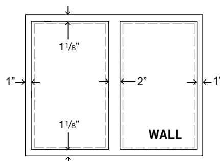
STANDARD OVERLAY - NO BUTT DOORS
