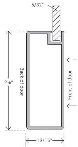
AF03 Frame Profile
