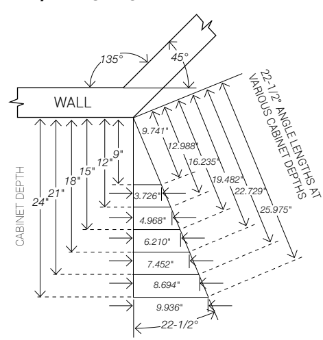
22 1/2° ANGLE CHART
