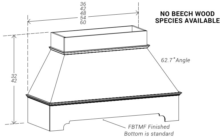
Overall Width Chart for Standard & Valance Compound Angle Hoods
