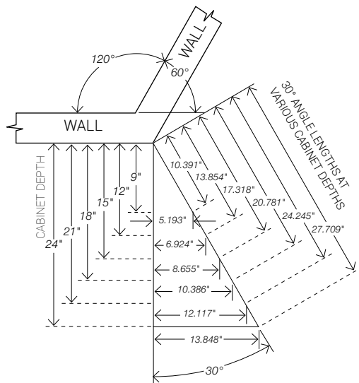
30° ANGLE CHART
