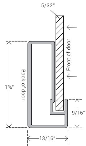
AF04 Frame Profile
