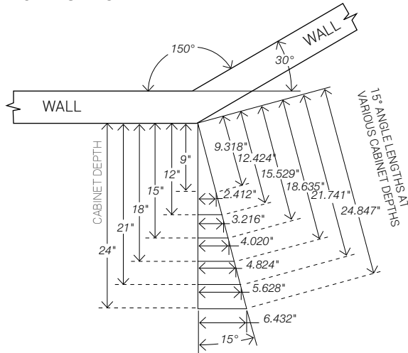
15° ANGLE CHART
