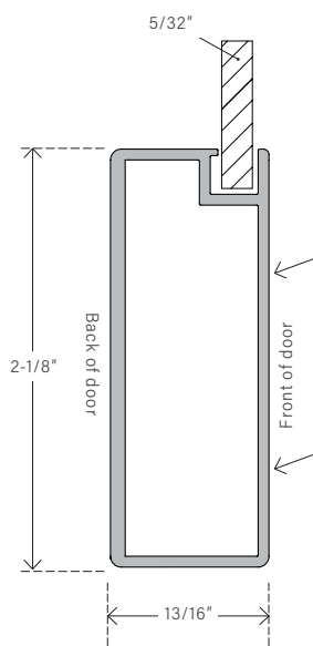
AF03 Frame Profile
