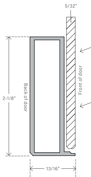
AF06 Frame Profile
