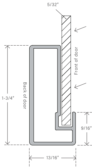
AF04 Frame Profile
