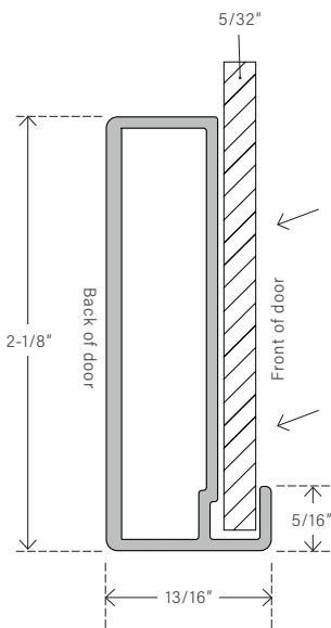
AF02 Frame Profile
